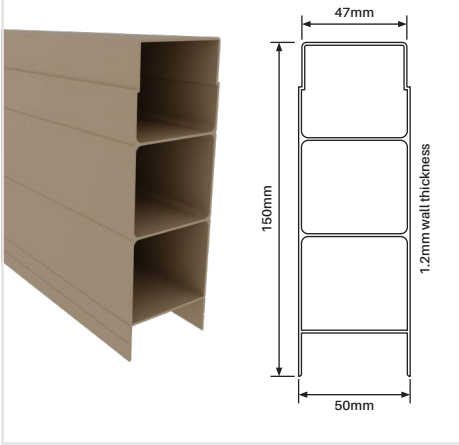
Stackable sleeper
